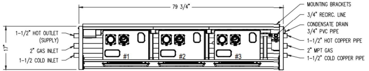
PLAN VIEW
